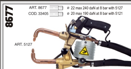
Water-cooled pneumatic gun. Standard and large gap arms item 5127+5137.
