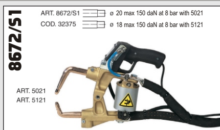
Smart gun: pneumatic gun with air and water cooling. Standard and large gap arms item 5001+5085 and item 5121+5185.
