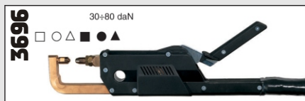
Hand-operated C type gun with air cooling. Reduced overall dimensions. Cables length 1600 mm.
